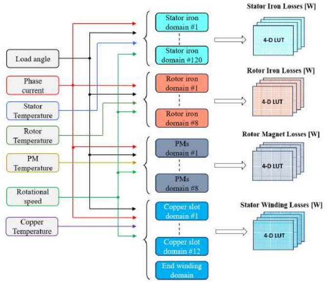
Fig. 3: Schematic losses structure of the EM model.
