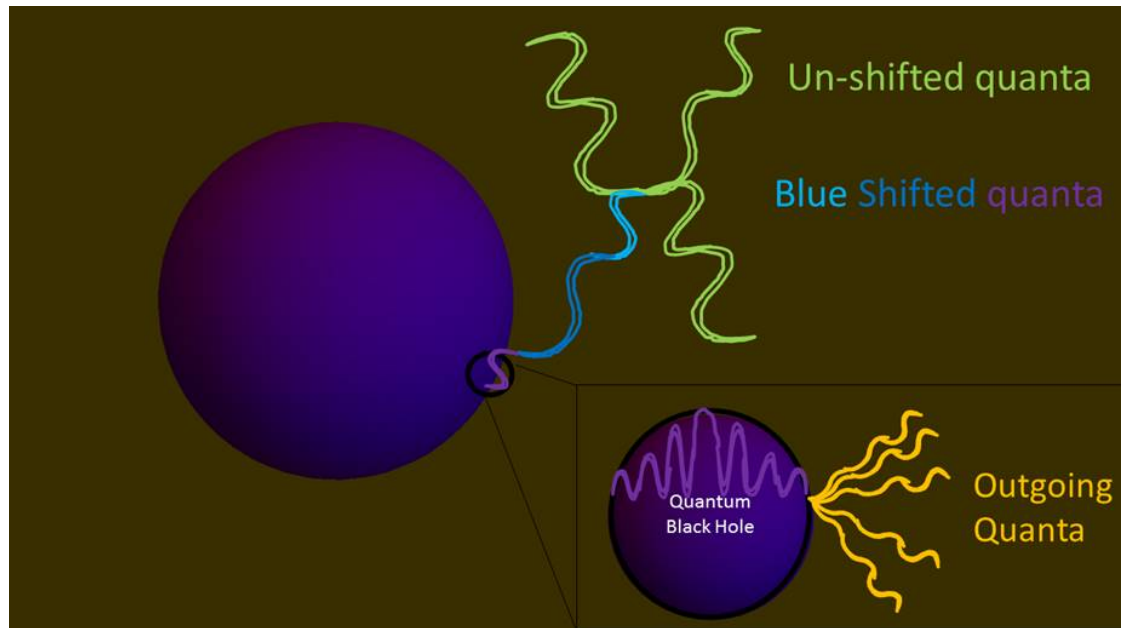
Figure 1: A simple view of Hawking radiation. A quantum, here represented as spin 2 bosons, interacts with another quantum and becomes entangled. One of the quanta falls into a black hole and as it falls it gains energy, the wavelength shortens and just as it hits the event horizon, it collapses into a quantum black hole. Inset, about one Planck time after the formation of this quantum black hole it decays via Hawking radiation into a thermal spectrum of quanta of all kinds at a very high temperature.
