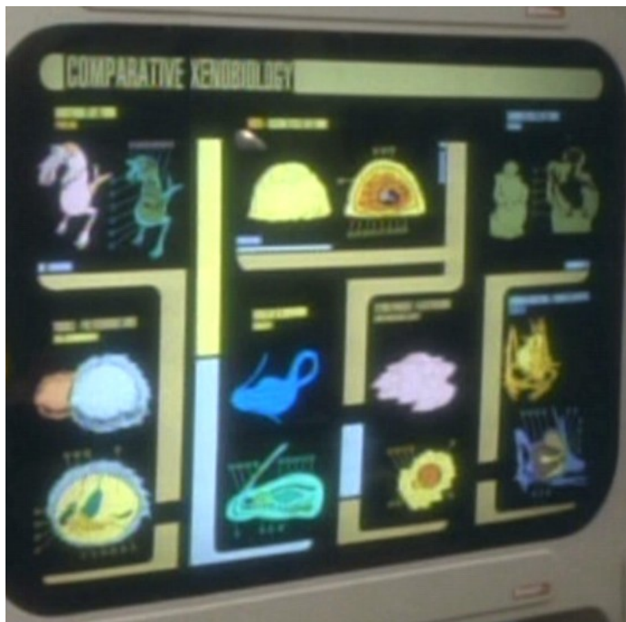
“Comparative Xenobiology” computer interface in a classroom. (Image: Star Trek: The Next Generation)
