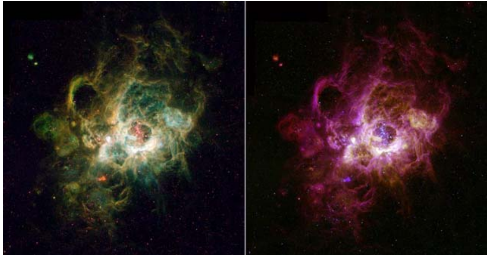
Emission nebula NGC 604, in the nearby galaxy M33. Color as published (left) and as the human eye would see it (right). (Image: Donald E. Davis)
