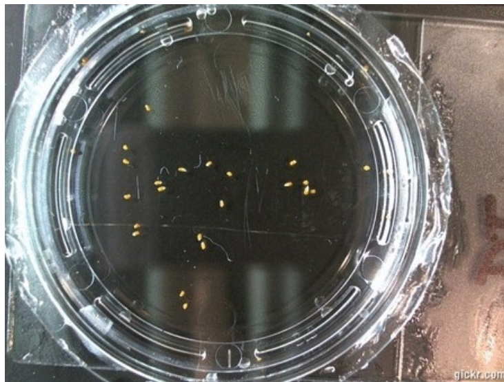
GROWTH OF TOBACCO SEEDS IN DI WATER.
