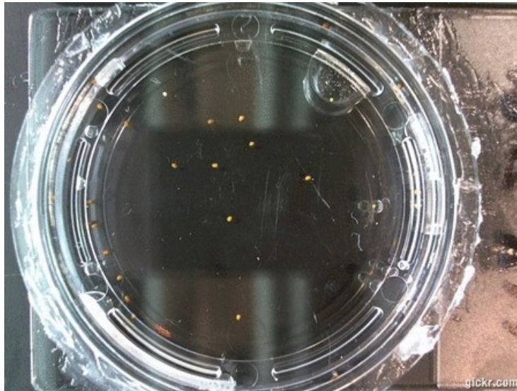
GROWTH OF TOBACCO SEEDS IN 66% D 2 O.
