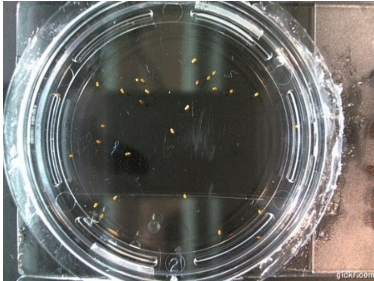
GROWTH OF TOBACCO SEEDS IN 33% D 2 O.
